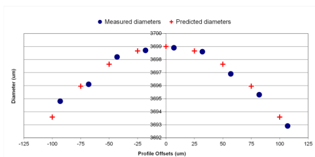
Figure 3. Diameter measurements (solid circle) from nine parallel traces at 25 \mu\text{m} increments through the central region of the Brinell indentation. Also shown are predicted diameter values (cross) based on a circular indentation.
