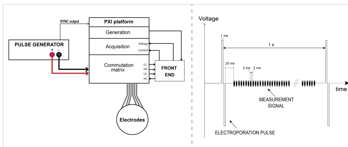
Fig. 2: Block diagram of the complete system and generated signals. Pulse generator creates biphasic electroporation pulses, the SYNC output is used for synchronization with the PXI system. After commutation of connections (25 ms delay) measurement signals are generated and acquired each 2 ms. 230 complete spectra are measured between consecutive pulses.
