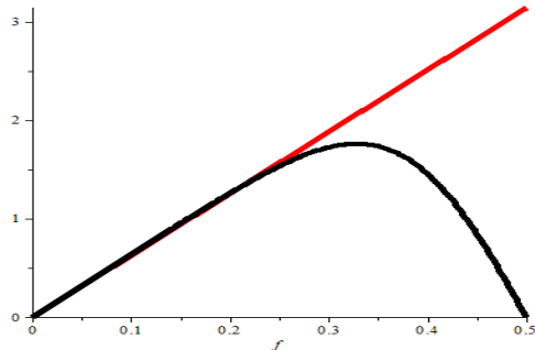
Figure 5. Magnitude of the frequency response of derivative operator based on cubic splines with 9 coefficients.
