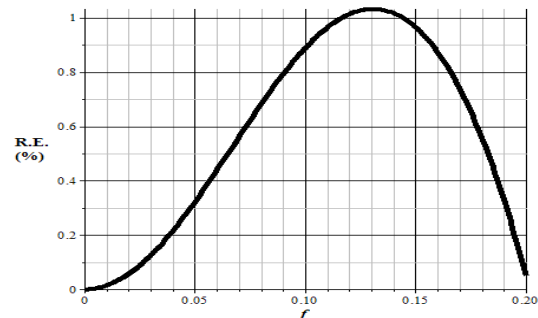
Figure 8. Relative error as a percentage between ideal response and cubic spline derivative operator with 9 coefficients.
